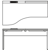
DESK - CURVED FREESTANDING X - 231 L 68 1/2" x 24"-36" x 30"
