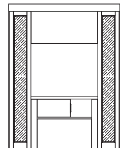
ADA TV DIVIDER WALL G-101-04A 73"W x 12"D x 95"H (assem)
