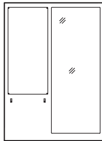
ENTRY ORGANIZER - ADA G-101-13.1 25"W x 20"D x 46.5"H
